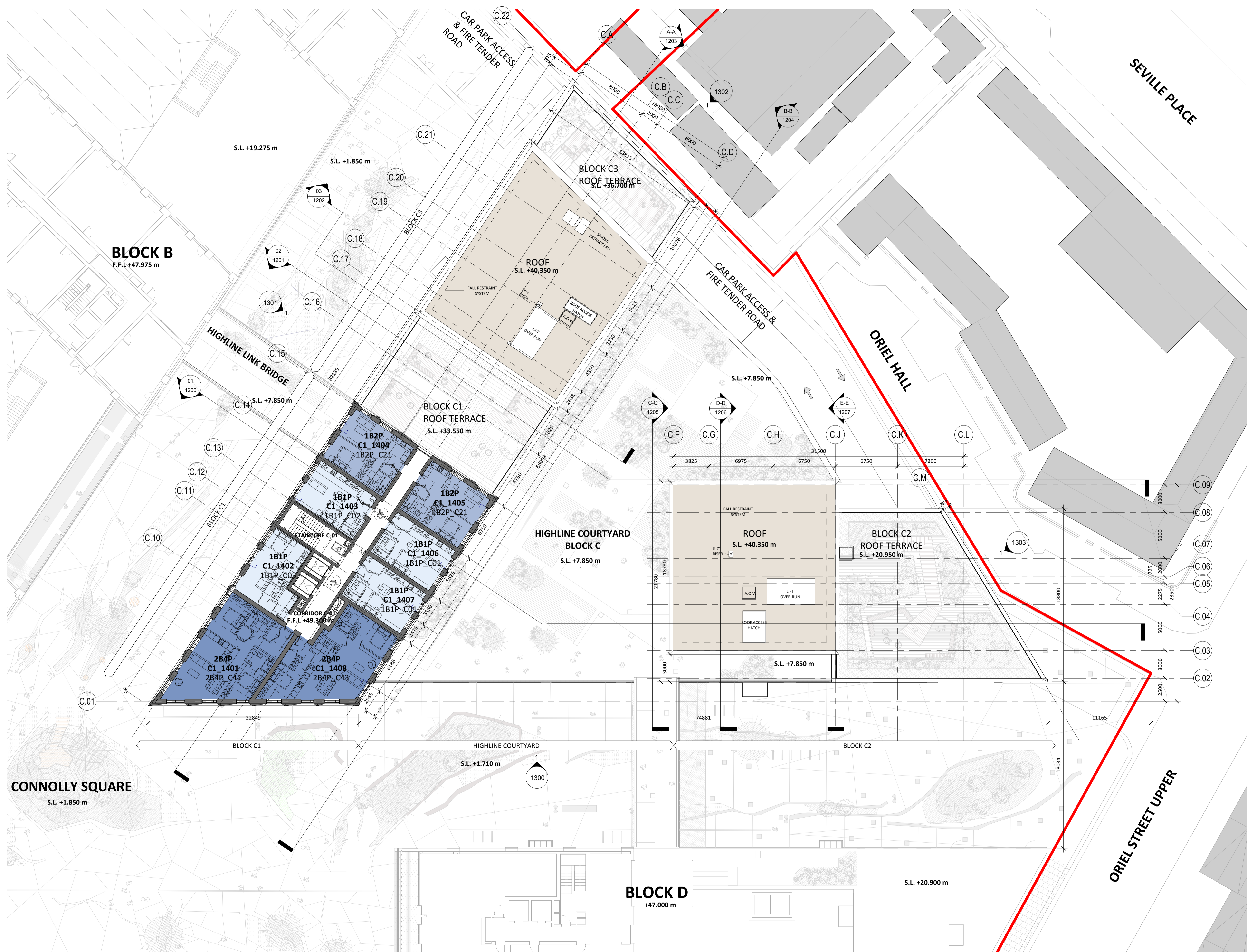
1 BLOCK C PLAN_LEVEL 14 1 : 200
